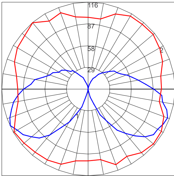
POLAR CANDELA PLOT (14W LED, 3000K/4000K)
